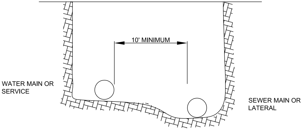
PARALLEL INSTALLATION
